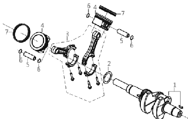
FIG.4 ROD,CRANKSHAFT CONNETING (E05)
