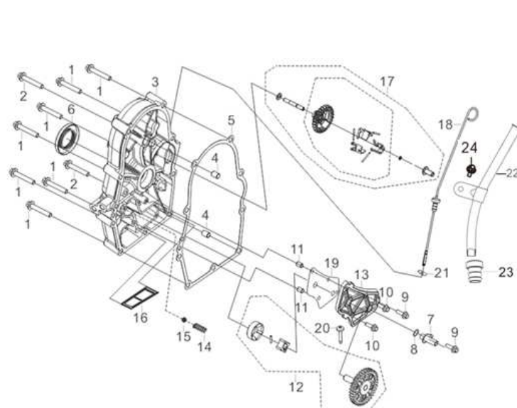
FIG.3 COVER SUBASSEMBLY, CRANKCASE / GEAR ASSY, GOVERNOR(E02)
