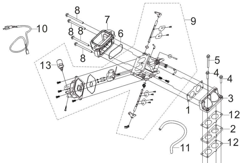
FIG.8 CARBURETOR ASSY. (E09)
