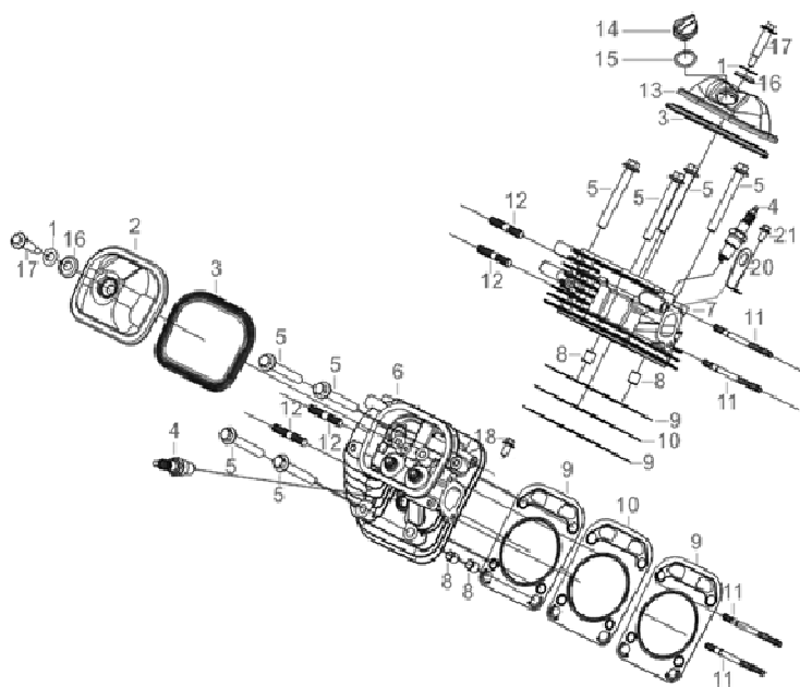
FIG.1 HEAD SUBASSEMBLY, CYLINDER / PLUG,SPARK(E03)
