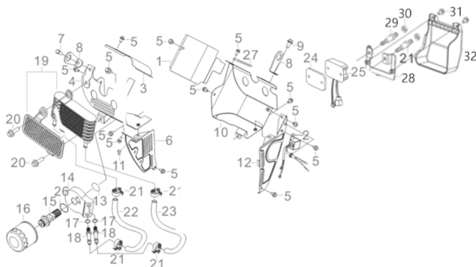
FIG.7 SHROUD, CYLINDER BODY / SHIELD,LOWER (E08)
