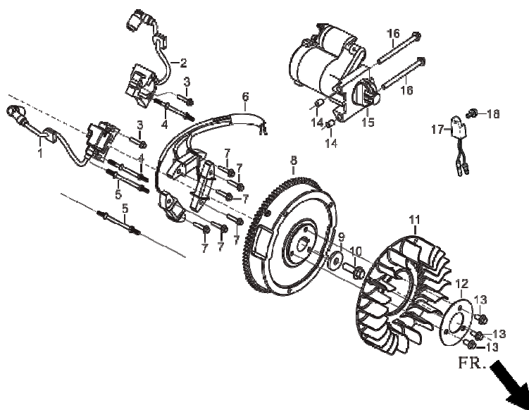
FIG.10 FLYWHEEL / IMPELLER / STARTER PULLEY / IGNITION COIL (E10)
