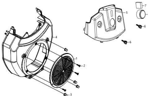
FIG.6 OUTER HOUSING (E07)
