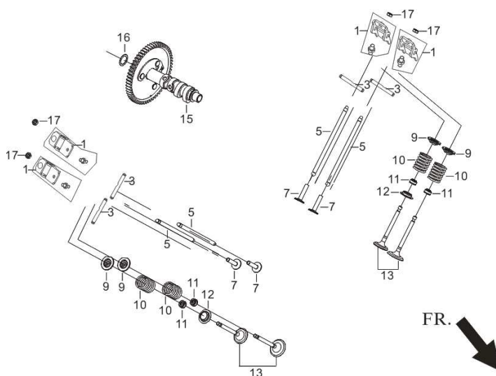
FIG.5 TRAIN,VALVE / CAMSHAFT SUBASSEMBLY (E06)
