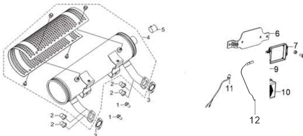
FIG.12 MUFFLER ASSY. (F02)
