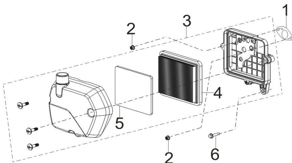
FIG.10 CLEANER, AIR
