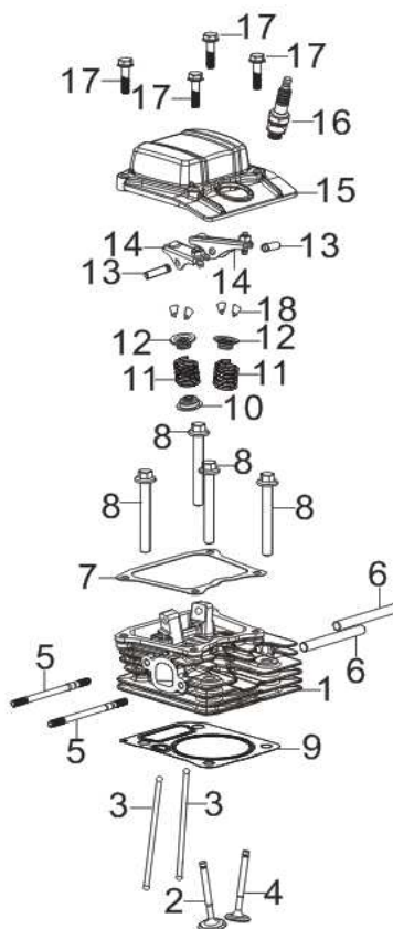
FIG.3 HEAD SUBASSEMBLY, CYLINDER / PLUG,SPARK
