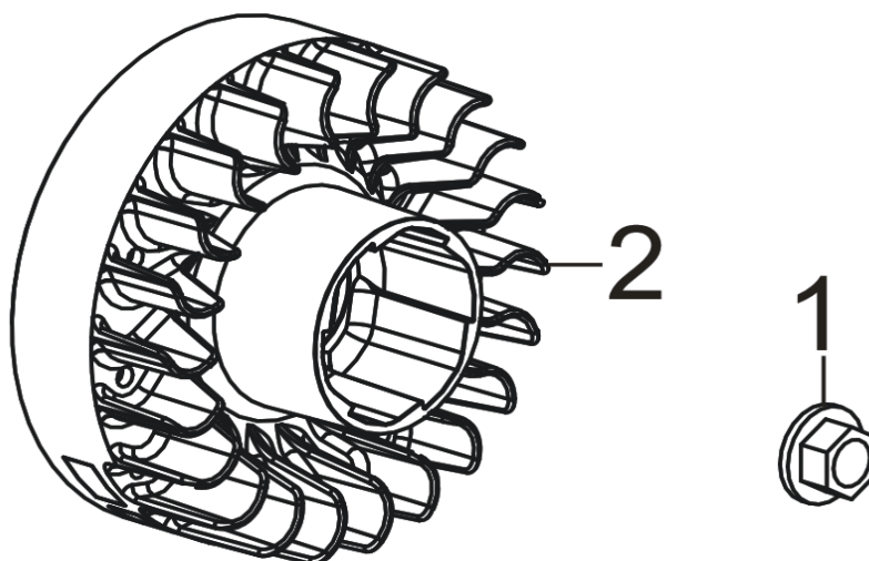
FIG.8 FLYWHEEL / IMPELLER / STARTER PULLEY / IGNITION COIL
