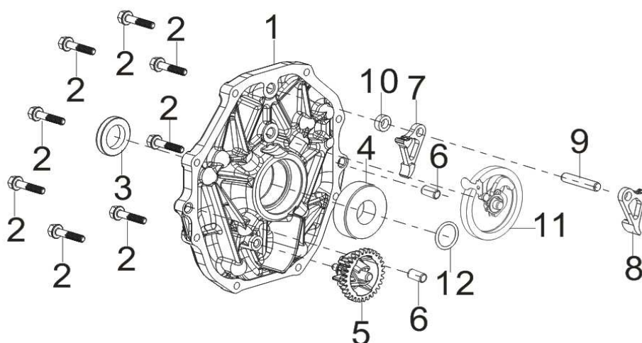
FIG.2 COVER SUBASSEMBLY, CRANKCASE
