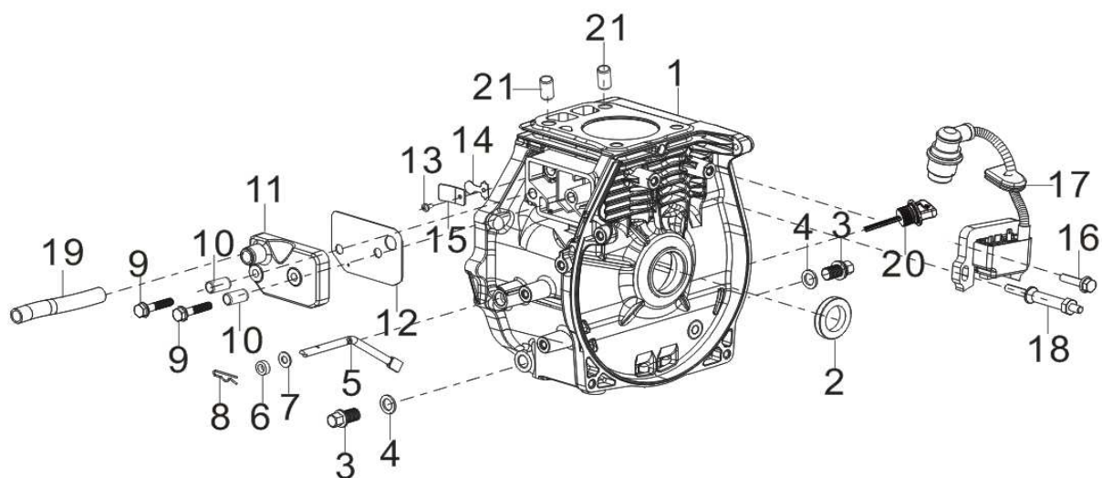
FIG.1 CRANKCASE. / GEAR ASSY, GOVERNOR.
