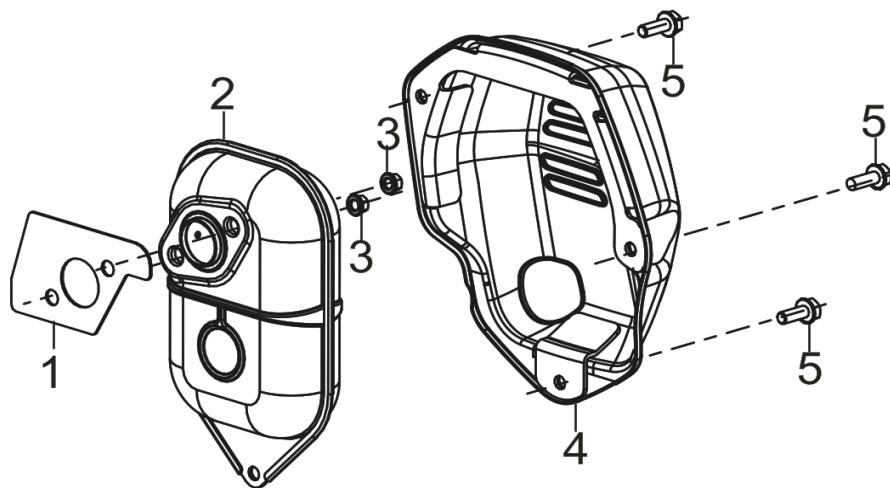
FIG.11 MUFFLER ASSY.
