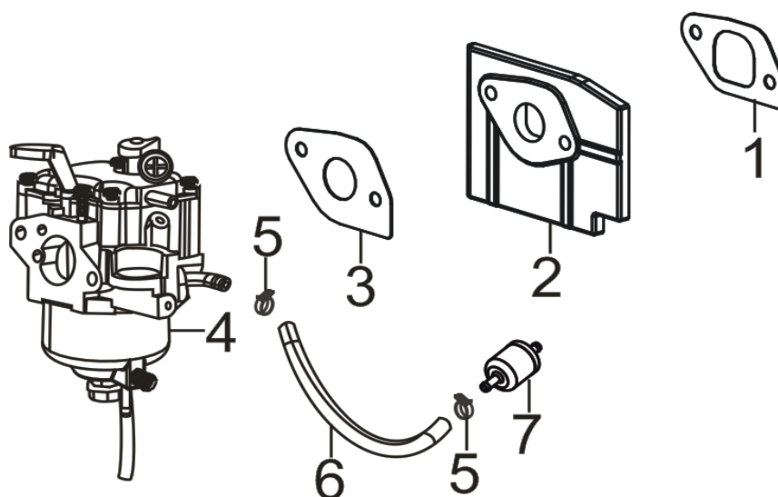
FIG.7 CARBURETOR ASSY.
