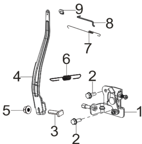
FIG.9 CONTROL ASSY, THROTTLE
