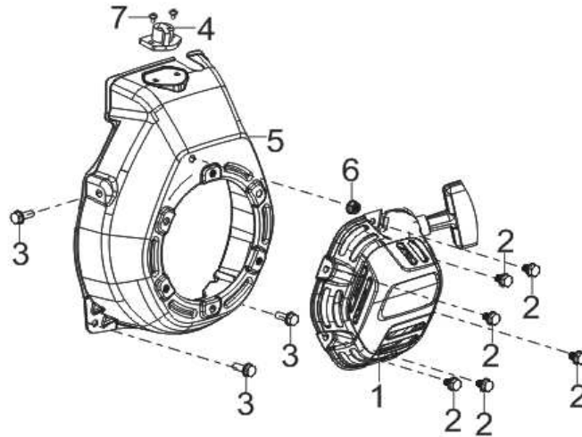
FIG.6 STARTER,RECOIL
