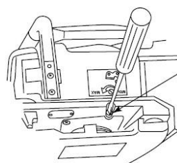
Chain oil flow adjusting
